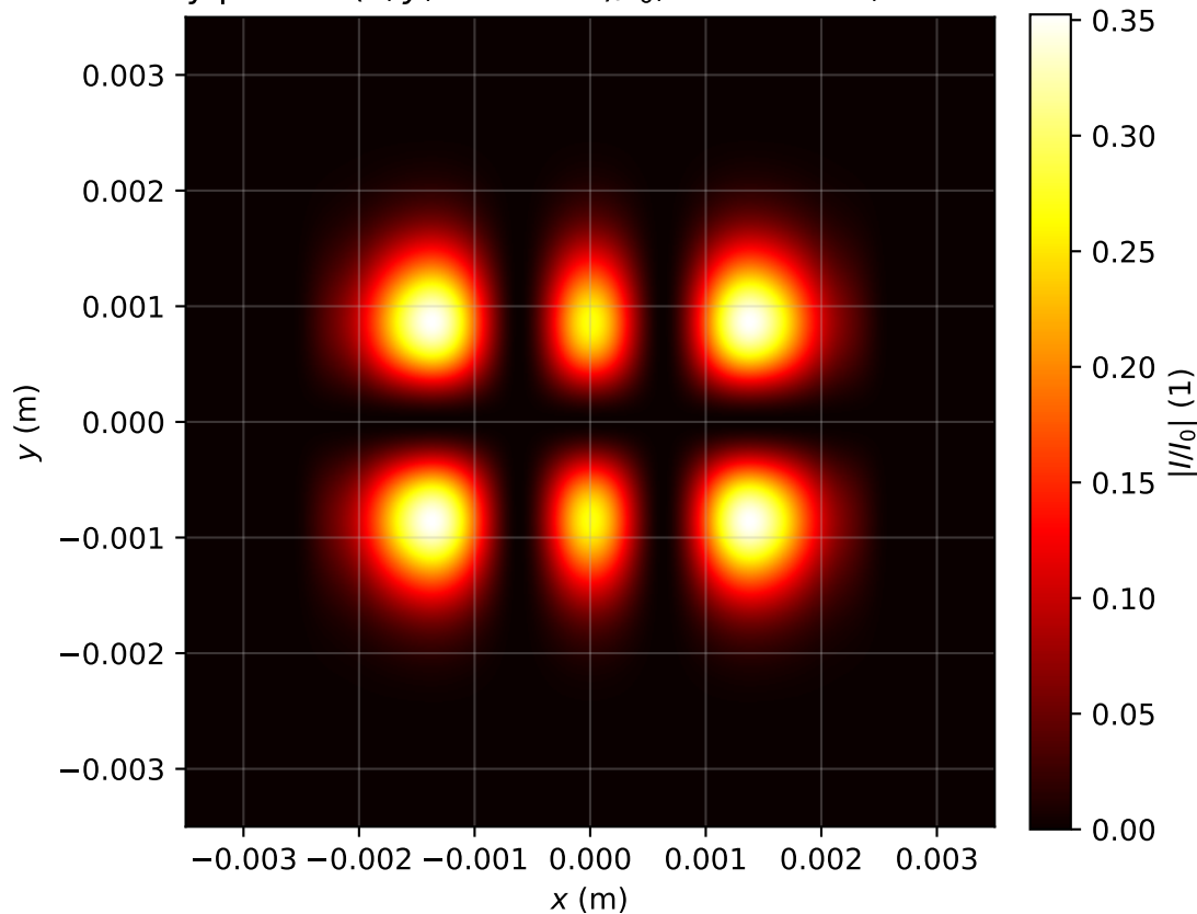
Intensity profile I(x, y, z = 2.866)/I_0 , P_{in}=0.5P_{cr} , artificial time
